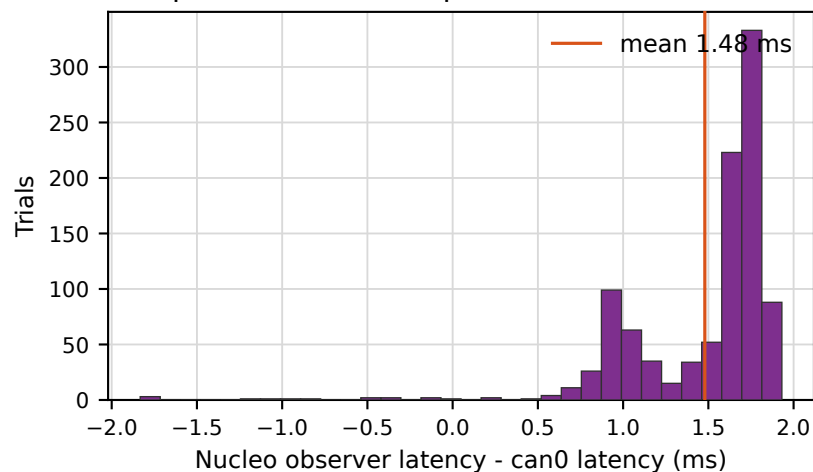
Independent timestamp offset distribution
