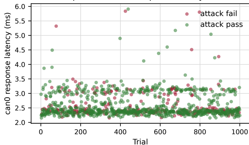
Baseline pass/fail with response delay
